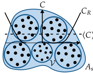
Figure 5.13: A schematic illustration of an agglomerate of PEM fuel cell carbon-supported catalyst particles with volume \mathcal{V} and surface area A_s . The black catalyst particles are surrounded by a carbon/ionomer/binder mixture. The dissolved oxygen concentration decreases from its value C_R at the particle surface towards the interior of the particle, due to the oxygen reduction reaction.
